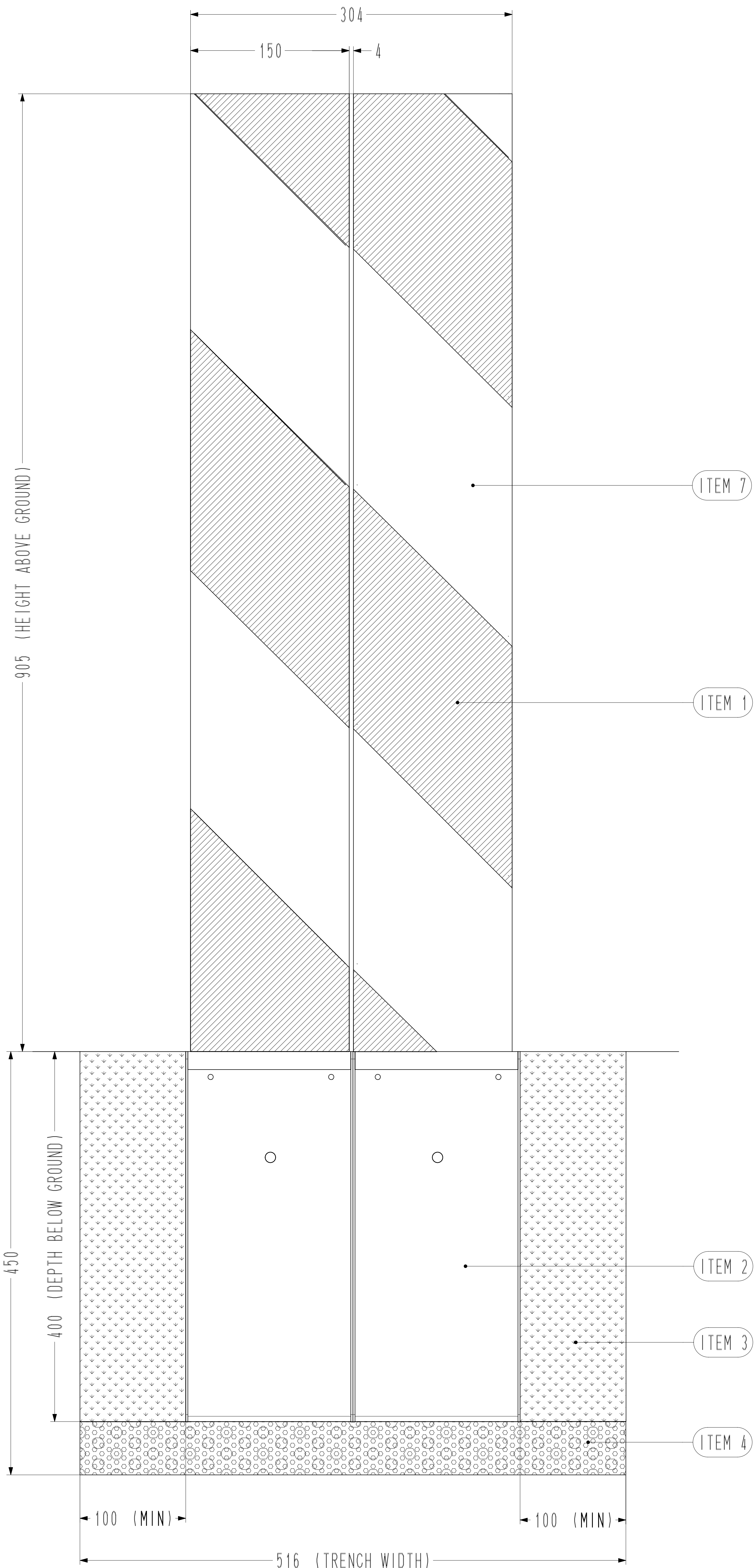
FRONT VIEW (LEFT HAND SIDE)
