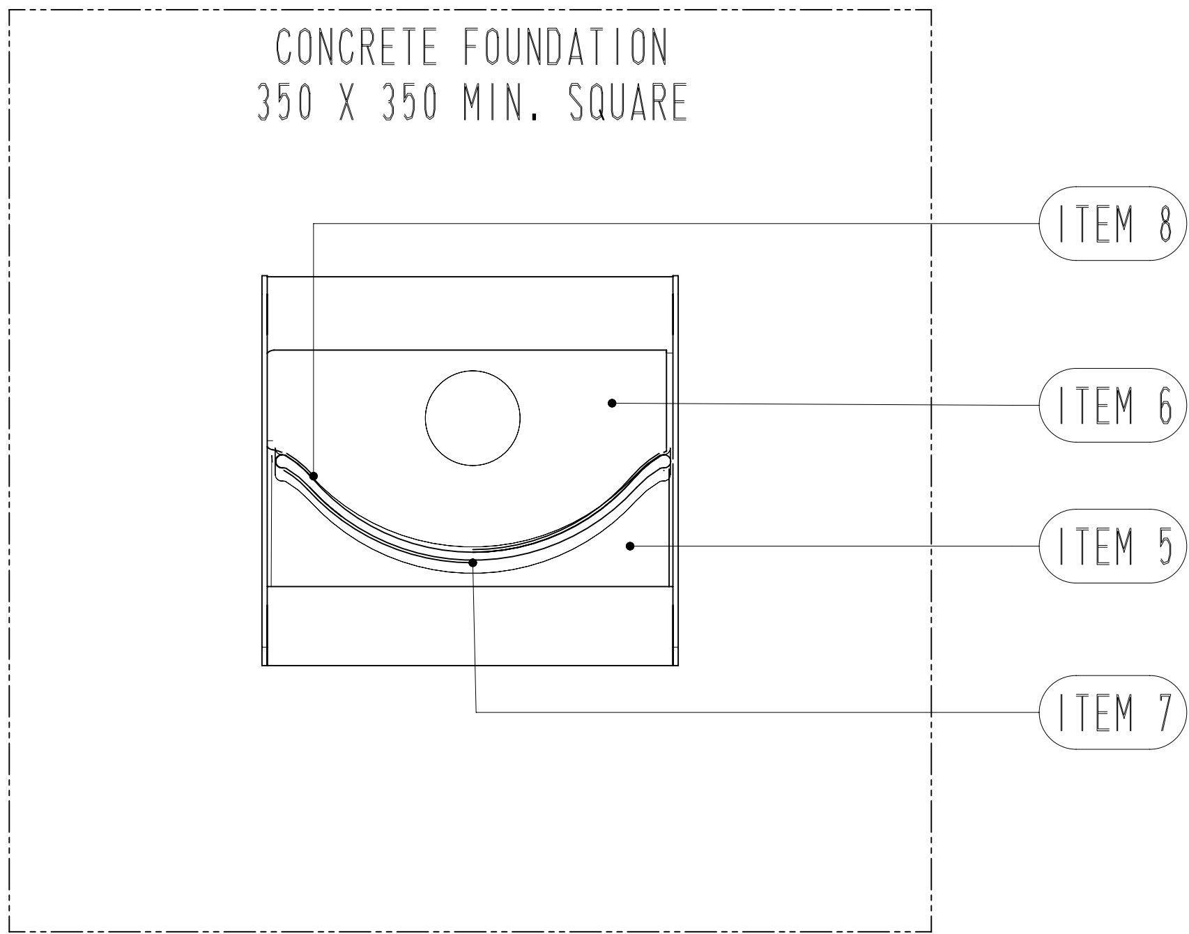
PLAN VIEW ( NEAR SIDE)
