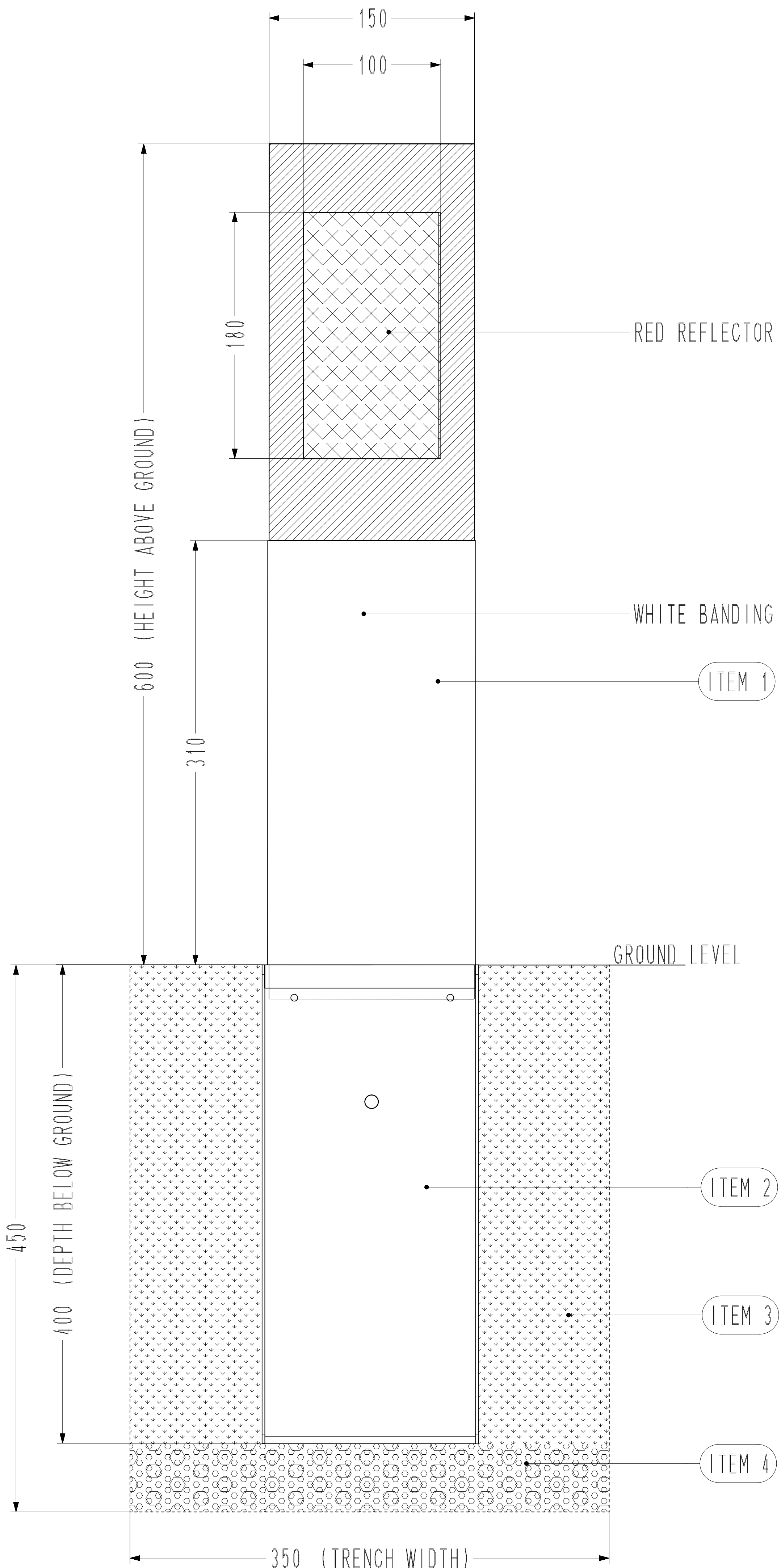
FRONT VIEW ( NEAR SIDE)
